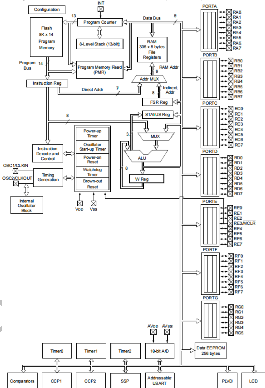
Figure 1.DIF81F964 BLOCK DIAGRAM
