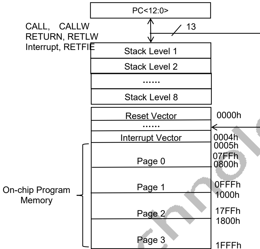
Figure 2. PROGRAM MEMORY MAP AND STACK FOR THE DIF81F964
