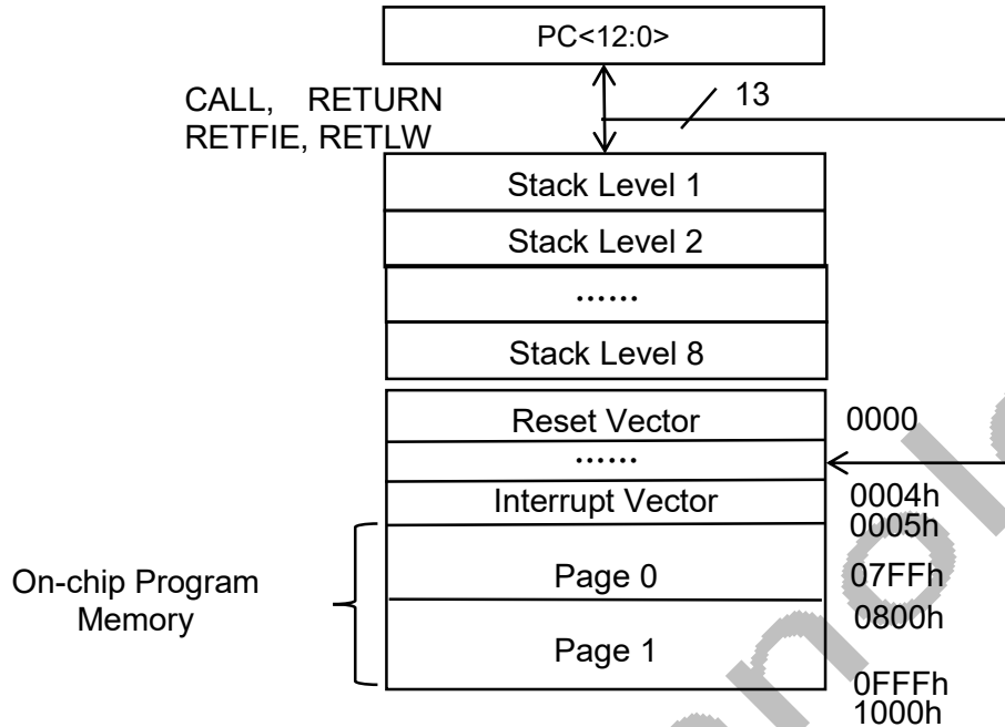
Figure 2. PROGRAM MEMORY MAP AND STACK FOR THE DIF81F901
