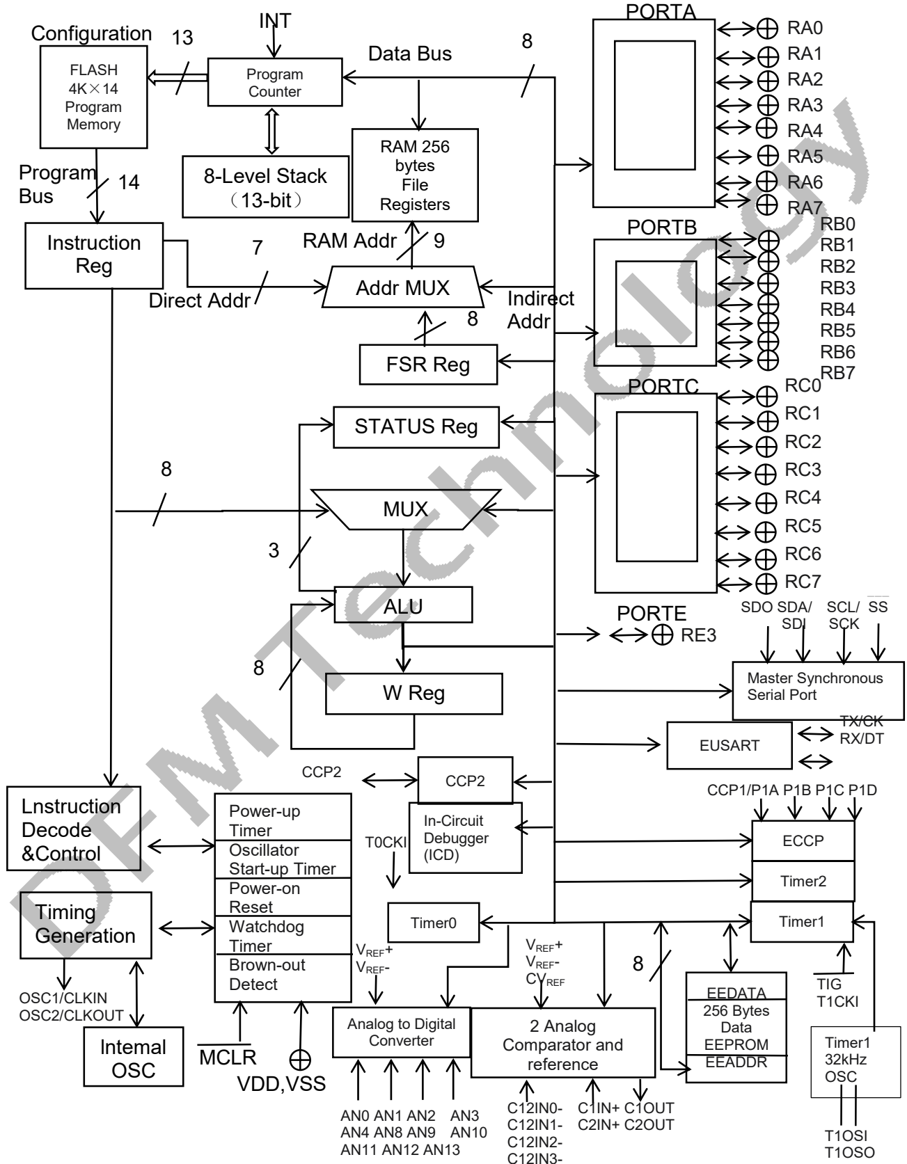
Figure 1. DIF81F901 BLOCK DIAGRAM
