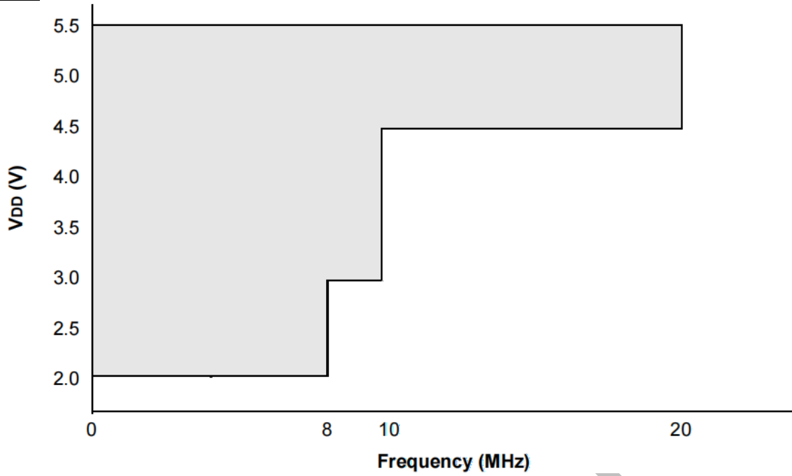
Figure 4. DIF81F901 VOLTAGE-FREQUENCY GRAPH, -40^{\circ}\text{C} \leq T_A \leq +125^{\circ}\text{C}
