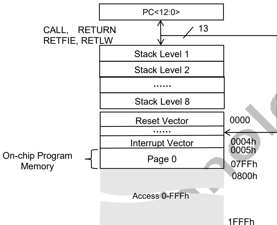
Figure 2. PROGRAM MEMORY MAP AND STACK FOR THE DIF81F705
