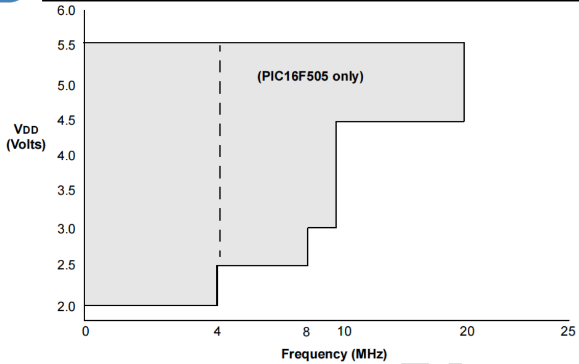
Figure 4.DIF80F527 VOLTAGE-FREQUENCY GRAPH, -40^{\circ}\text{C} \leq T_A \leq +125^{\circ}\text{C}
