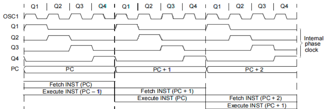
Figure 2.CLOCK/INSTRUCTION CYCLE
