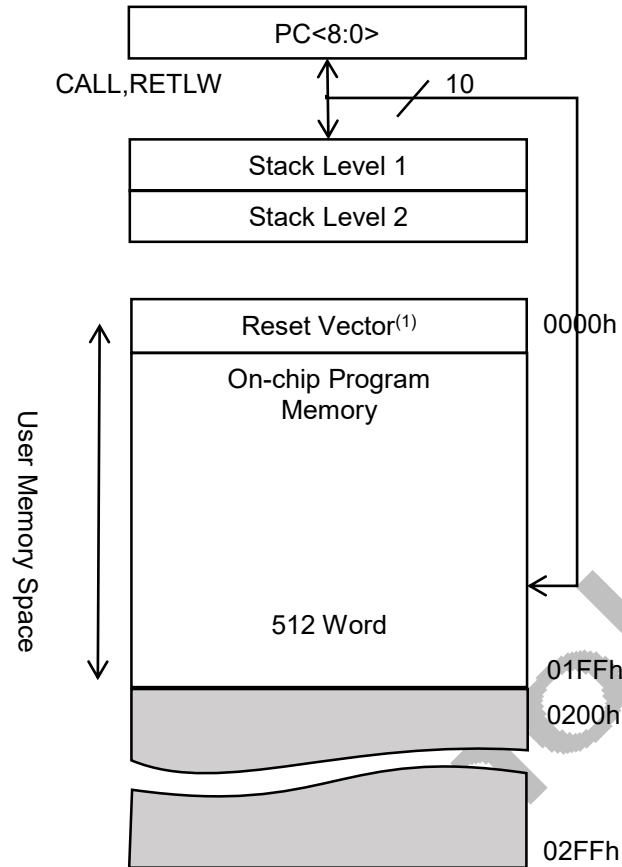
Figure 3. PROGRAM MEMORY MAP AND STACK FOR THE DIF80F224
