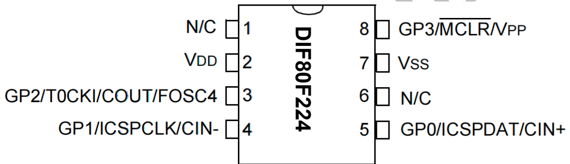
DIF80F224DI( 8-pin DIP)
