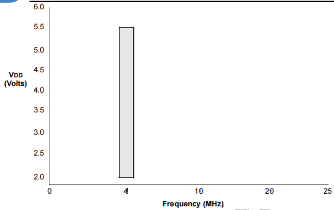
Figure 4. DIF80F224 VOLTAGE-FREQUENCY GRAPH, -40^{\circ}\text{C} \leq T_A \leq +125^{\circ}\text{C}
